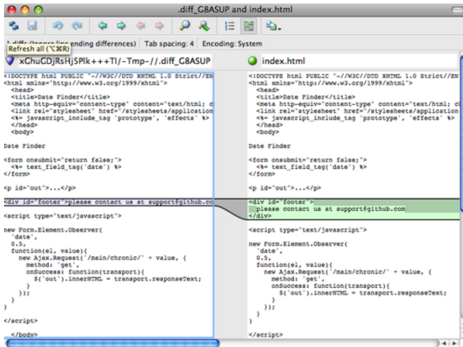
Figure 7.1: P4Merge
