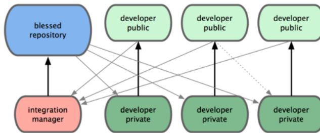
Figure 5.2: Integration-manager workflow
