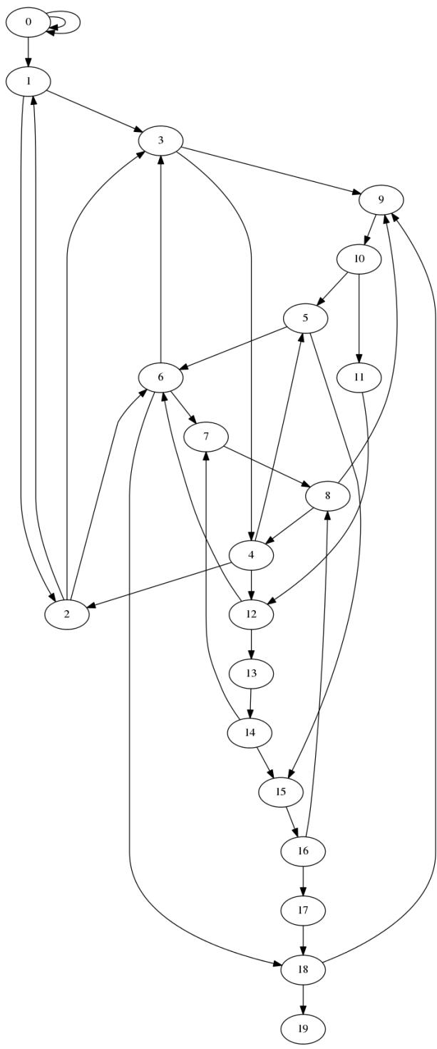
Figure 5: The full graph 338
